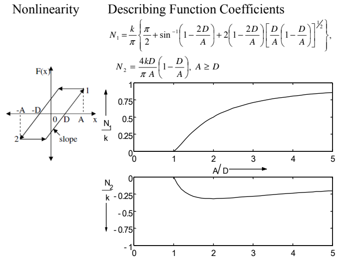
Fig. 2. LHS governor dead-band (backlash) nonlinearity and RHS Fourier series coefficients of governor dead-band.
