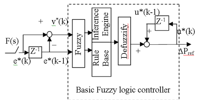
Fig. 4. A typical Fuzzy based load frequency controller (FLFC) for an AGC.
